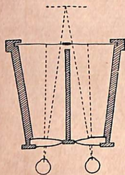
FIG. 50. Plan of Brewster's Refracting Stereoscope, old model. — D. Brewster, The Stereoscope, its History, Theory and Construction , 1856.
