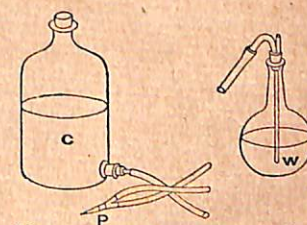
FIG. 21. Apparatus for the investigation of the temperature senses. C , cold; W , warm water; P , metal point.
