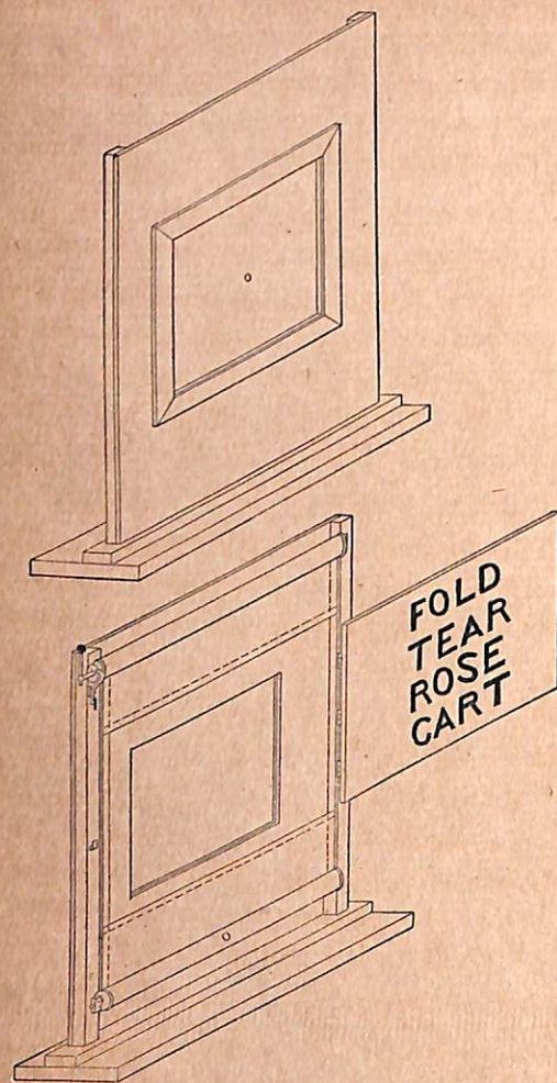
FIG. 42. Demonstrational Tachistoscope. A black curtain, mounted on strong spring rollers, is stretched behind a square opening in a black wooden screen. The upper Fig. (front) shows the curtain and the white fixation-mark. The lower Fig. (back) has the card-carrier thrown back to show the square opening in the curtain itself.
