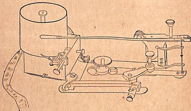
FIG. 37. Von Frey's Sphygmograph. The entire apparatus is bound upon the wrist, the button at the extreme right resting on the artery. The movements of the writing-lever are recorded on a very small, light drum, driven by a clockwork which is housed in the square box to the left. The clockwork also actuates a time-marker, shown in the Fig. at the lower edge of the drum.
