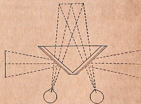
FIG. 49. Plan of Wheatstone's Stereoscope.
