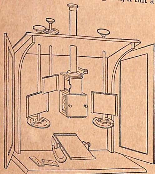
FIG. 10. Hering's Apparatus for the Investigation of Partial Colour Blindness.
