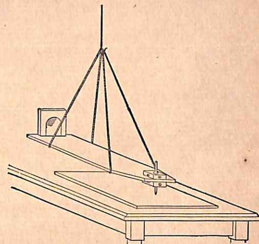
FIG. 34. Automatograph.
