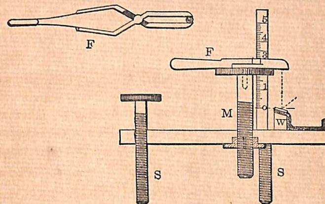
FIG. 26. Acoumeter for determining the Stimulus Limen of Noise. SS, set-screws (two of the three are shown), supporting a wooden platform. M, micrometer screw at the centre of the platform, with scale beside it. FF, spring forceps, lying on the head of M, and carrying a small shot for dropping on the glass plate above W. The shot rebounds, and falls noiselessly into a padded trough.
