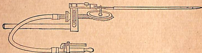
FIG. 29. Marey tambour (rubber-faced funnel) with writing lever, rubber tubing, and air-cock. The tubing is continued from the air-cock to the tambour on the wrist.
